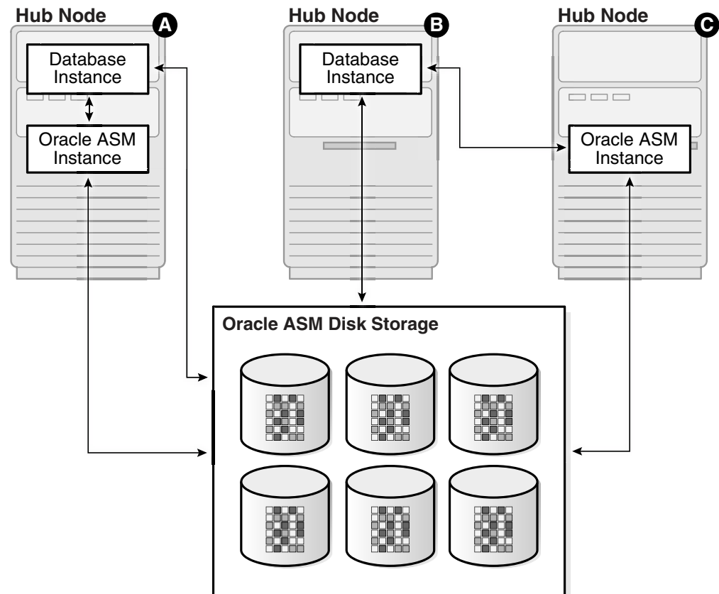
Figure 11-1 Oracle Flex ASM Client Configurations
